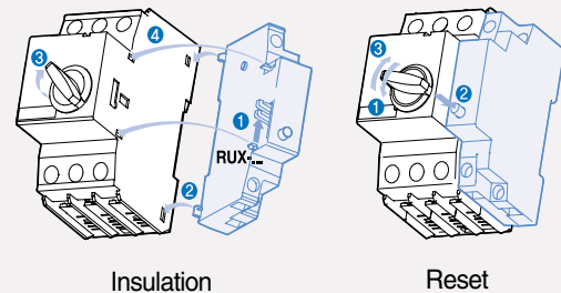
Insulation barrier
