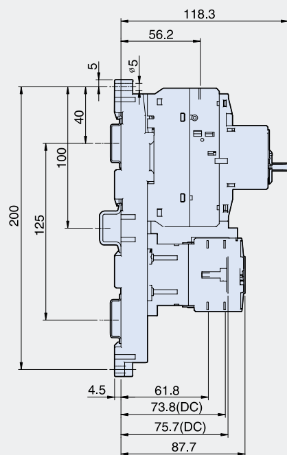
MMS-32H+GMC(D)-6M~16M
