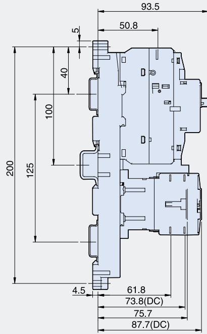
MMS-32S+GMC(D)-6M~16M
